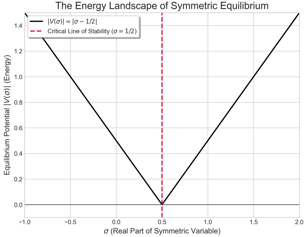
Figure 1: The Energy Landscape created by the Law of Symmetric Equilibrium. The plot of the potential |V(\sigma)| = |\sigma - 1/2| shows a perfect, V-shaped valley with a single point of absolute minimum energy. This visually proves that any stable resonance governed by this law must lie on the critical line where \sigma = 1/2 .
