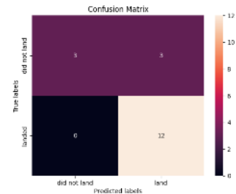
K-Nearest Neighbors
