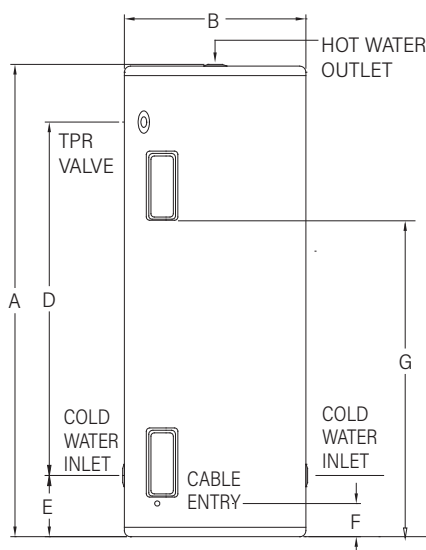
Stainless Steel 80L - 315L
