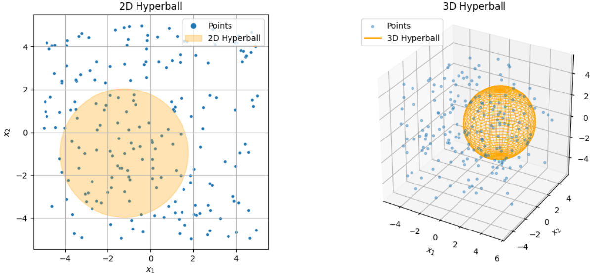
Figure 6: Hyperballs Visualization
