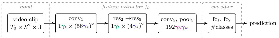
Figure 2: X3D as a video feature extractor followed by a linear classifier. The shape below each stage is its output size, following Table 1 . In the input stage, T_0 is the total frames in the raw video input and 3 implies each video’s frame is in RGB color space.
