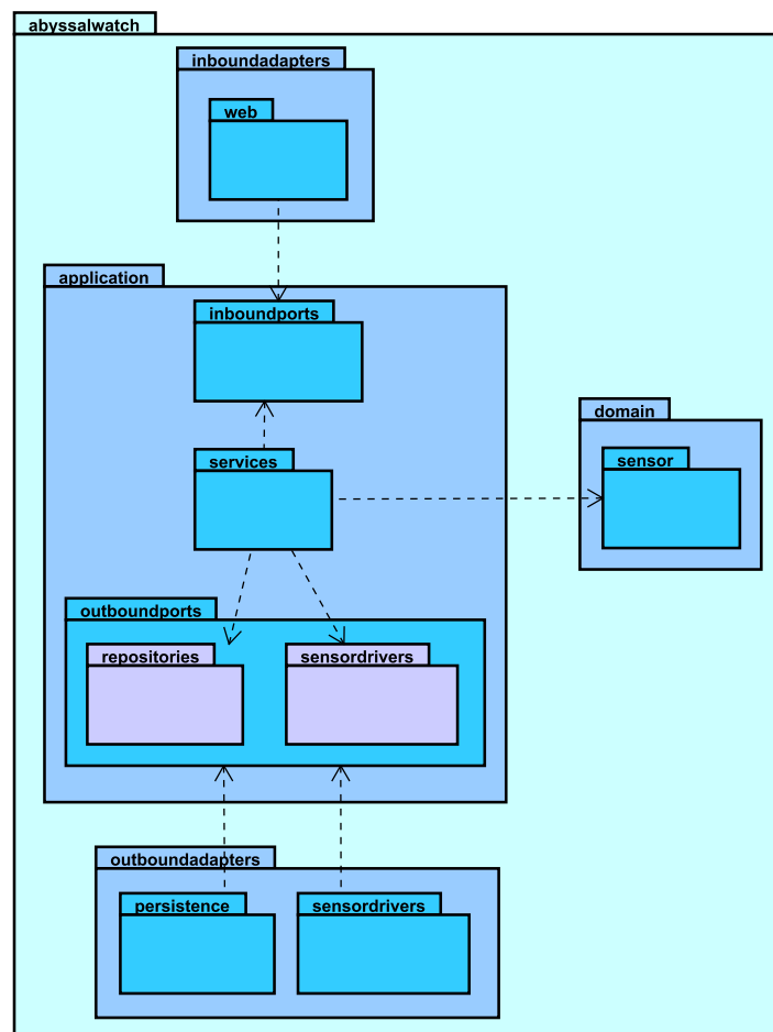
Figure 2.13: Package diagram of the application.
