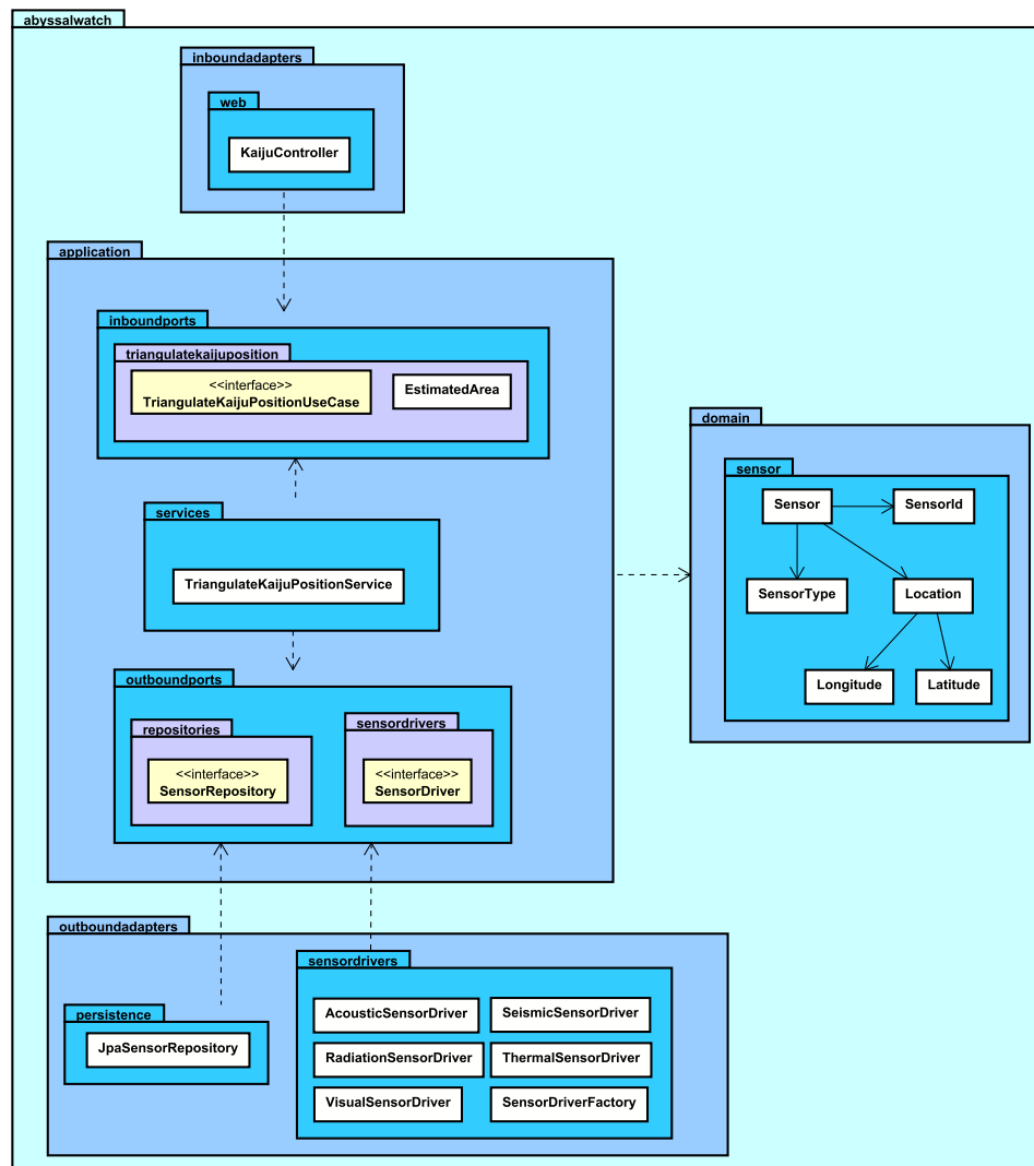
Figure 2.14: Package diagram of the application.
