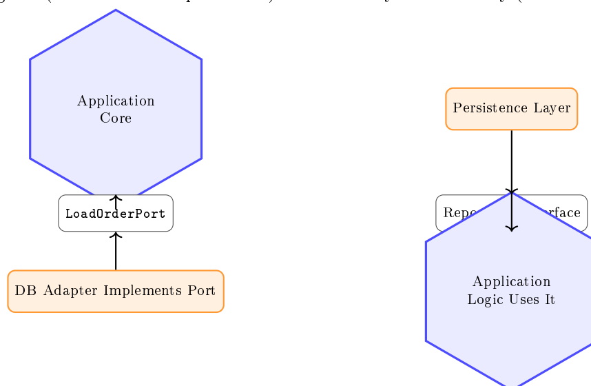
Figure 1.8: Contract ownership comparison: core-defined required ports vs provider-defined interfaces.
