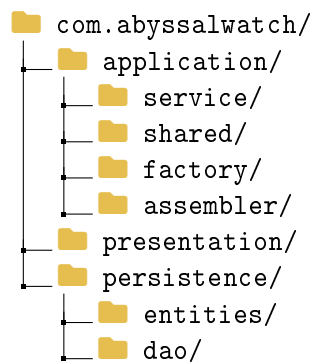
Figure 1.3: Business layer sub-packages when the flat service package is no longer enough.
