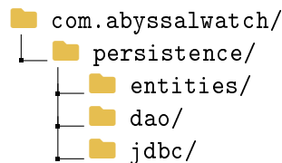
Figure 1.2: Entity types nested under the data access layer, closest to the database.
