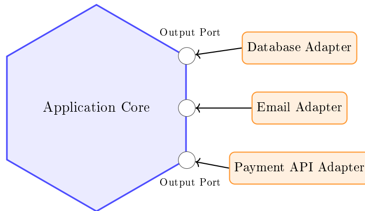
Figure 1.5: Driven adapters implement output ports for infrastructure concerns.
