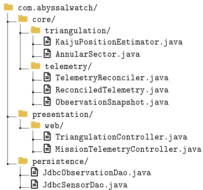
Figure 2.7: Simple FCIS layout: core plus delivery controllers with direct infrastructure access.
