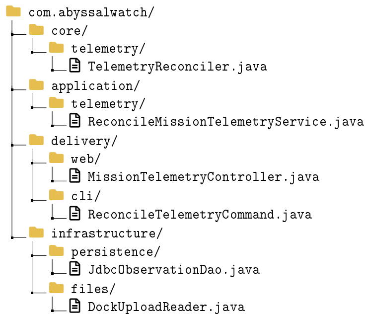
Figure 2.8: Evolved FCIS layout: delivery, application service, and infrastructure.
