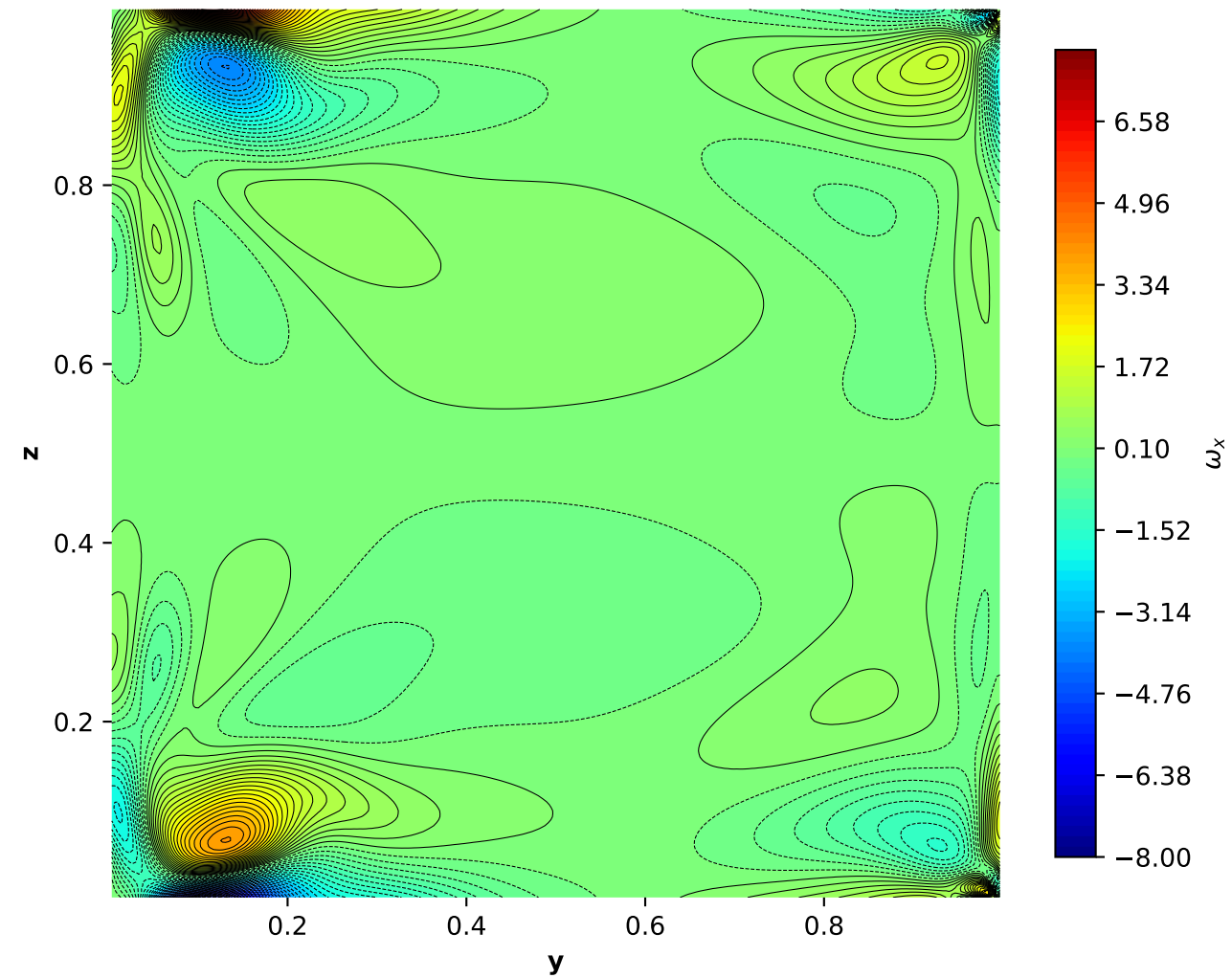
(a) Contours of \omega_x at (y,z)-symmetry plane Min = -9.16, Max = 9.16
