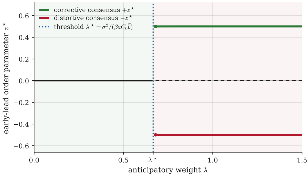
Amplification bifurcation of the early-lead order parameter
