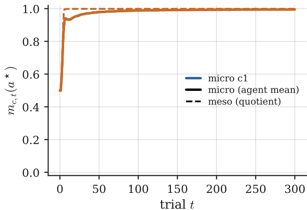
Two communities: efficient
