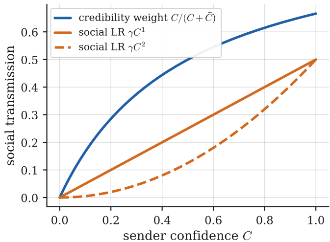
(b) credibility as network weight
