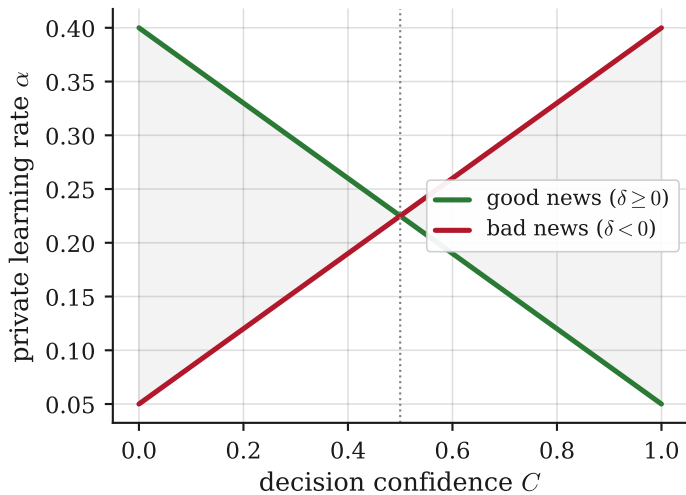
(a) confidence-gated learning rate
