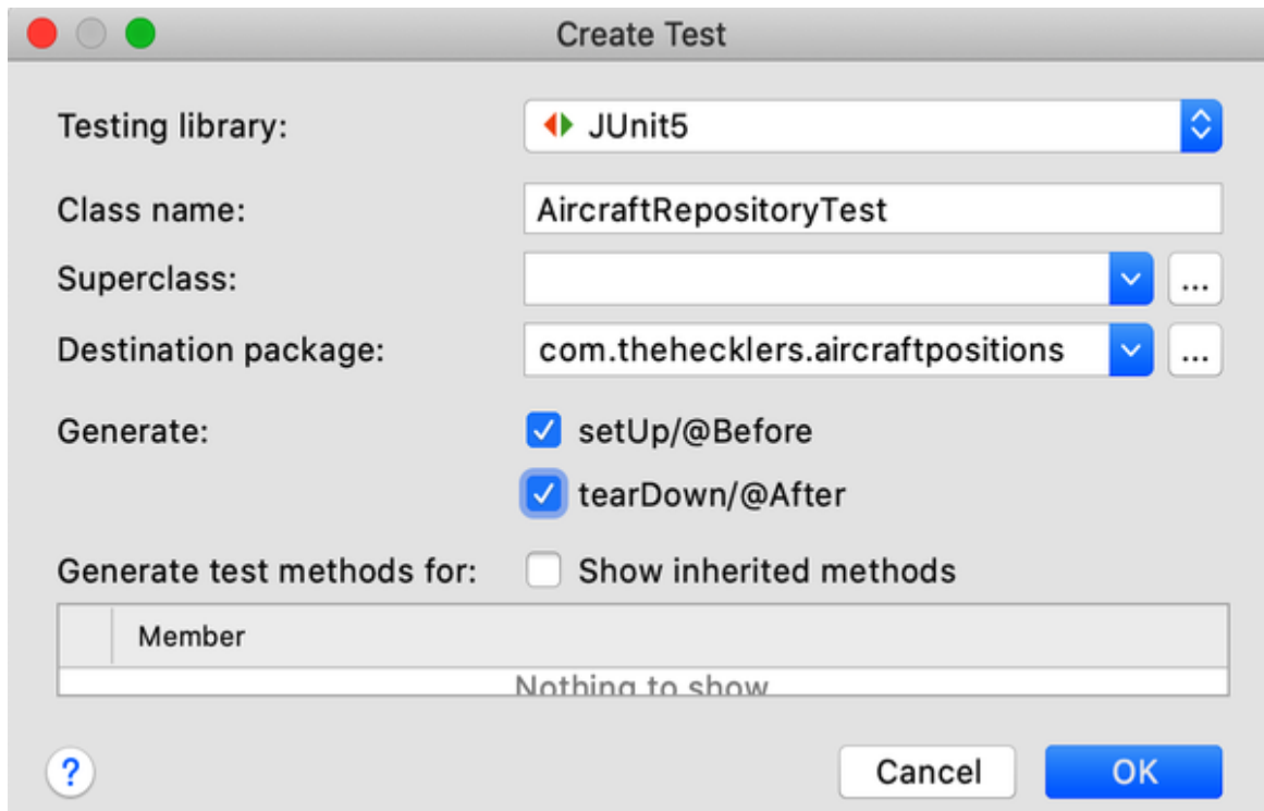
Figure 9-5. Create Test popup for AircraftRepository
