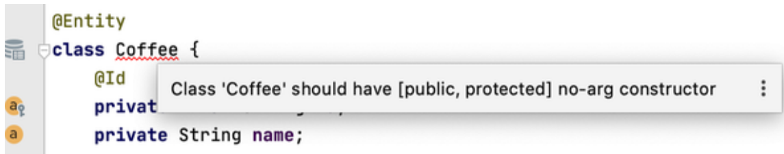
Figure 4-1. Missing constructor in the JPA Coffee class
