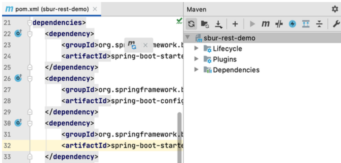
Figure 5-9. Reimporting project dependencies
