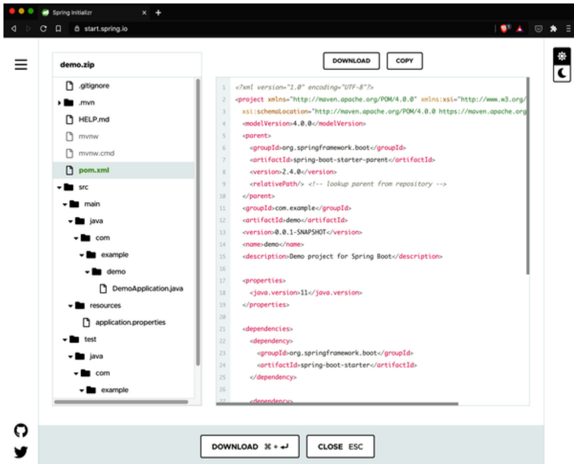
Figure 2-3. Spring Initializr's Project Explorer
