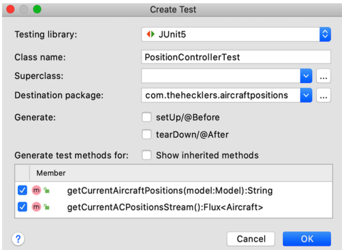
Figure 9-2. Create Test popup with Desired Options Selected
