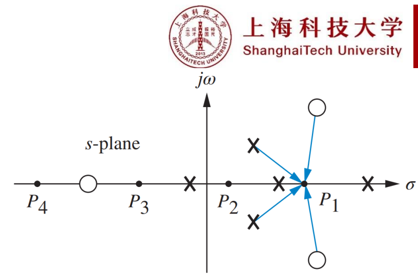
FIGURE 8.8 Poles and zeros of a general open-loop system with test points, P_i , on the real axis
