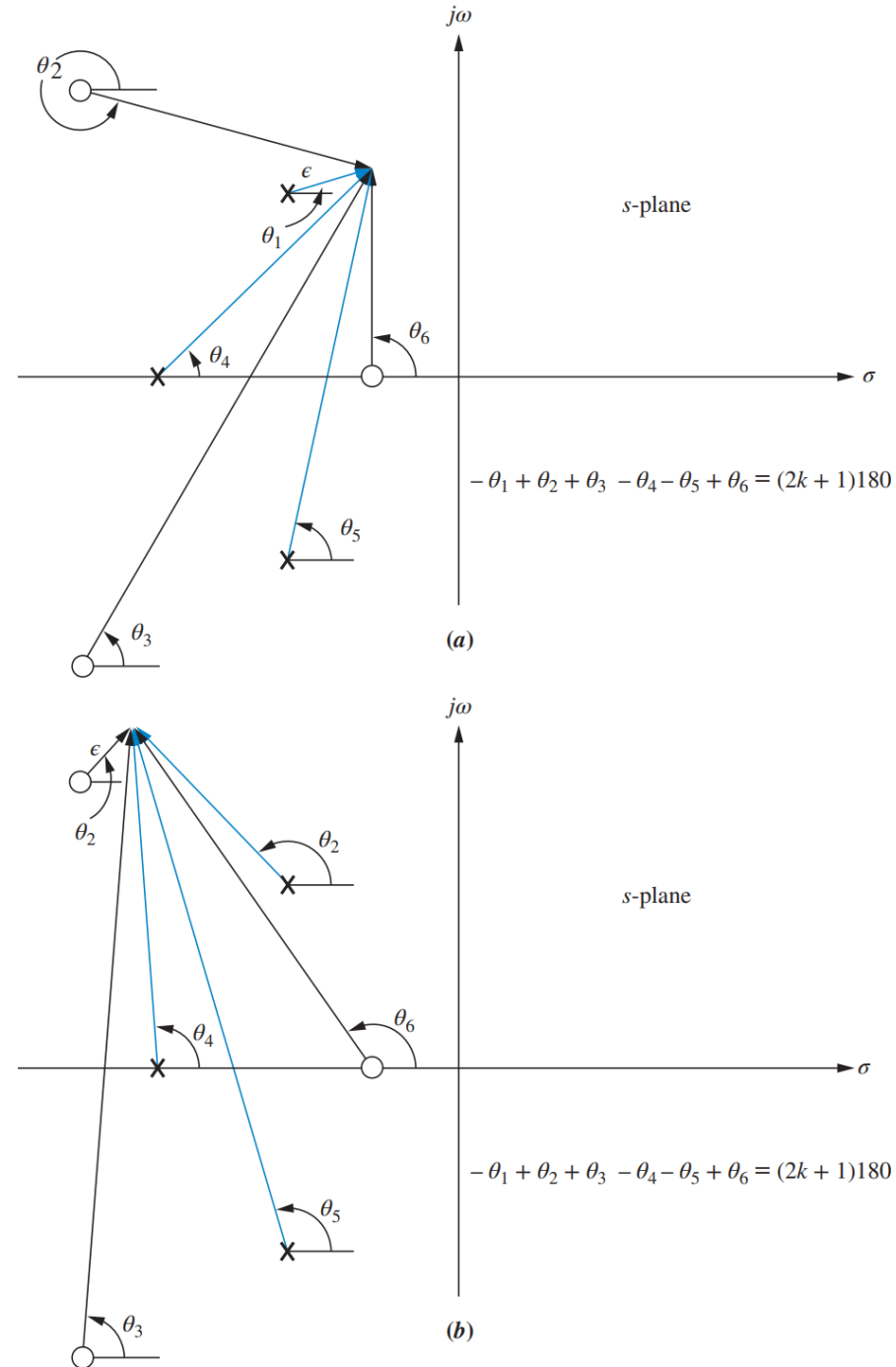
FIGURE 8.15 Open-loop poles and zeros and calculation of a. angle of departure; b. angle of arrival
