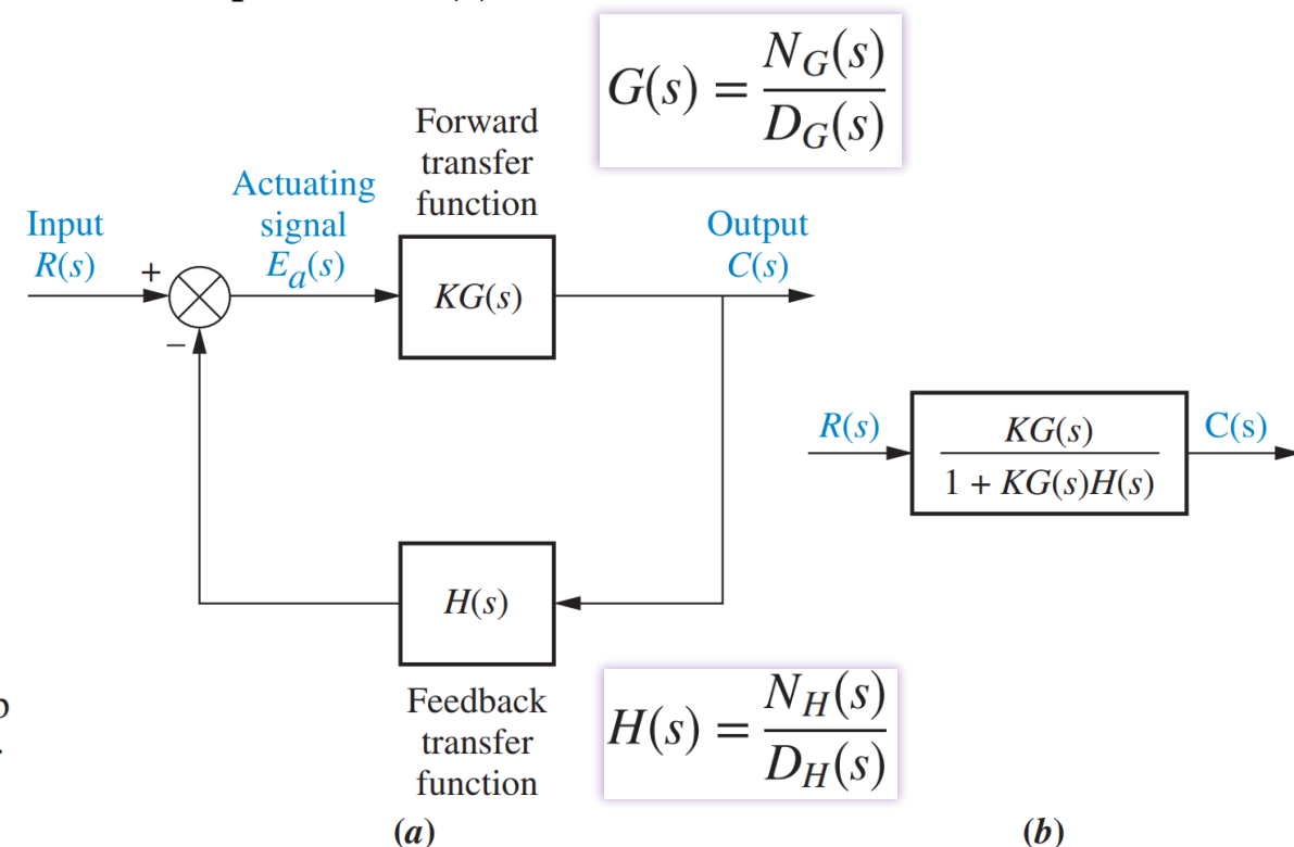
FIGURE 8.1 a. Closed-loop system; b. equivalent transfer function
