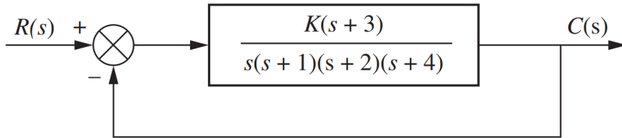
FIGURE 8.11 System for Example 8.2
