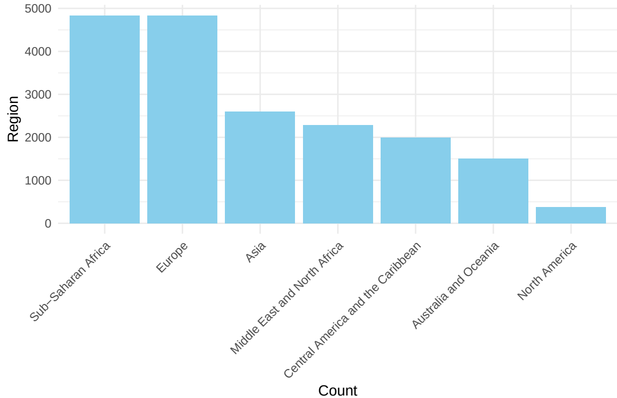
Frequency of Region
