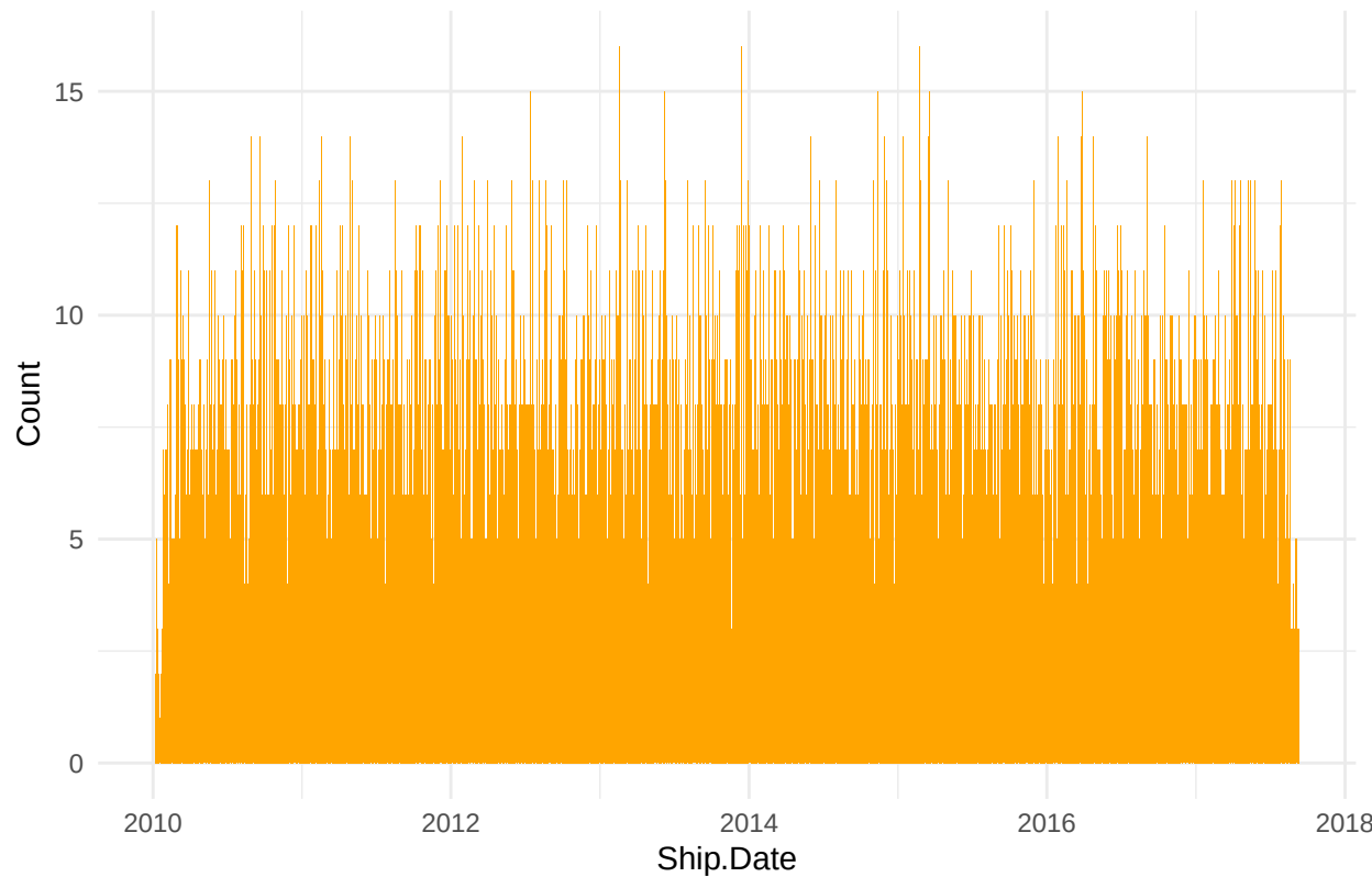
Frequency of Sales by Ship.Date
