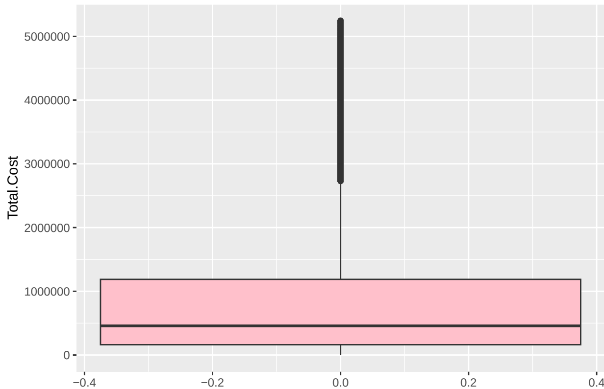
Boxplot of Total Cost
