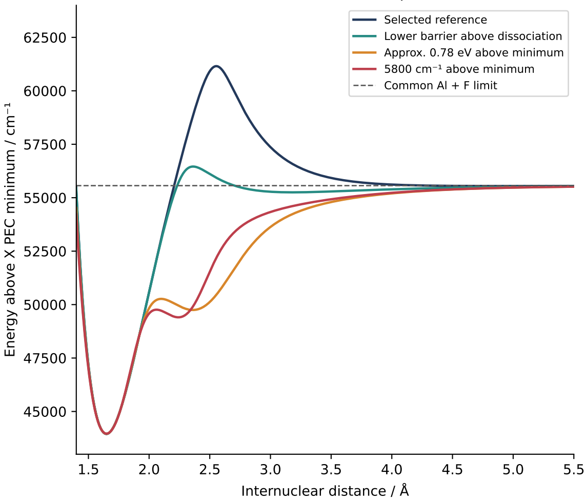
Lower local barriers create deep outer wells
