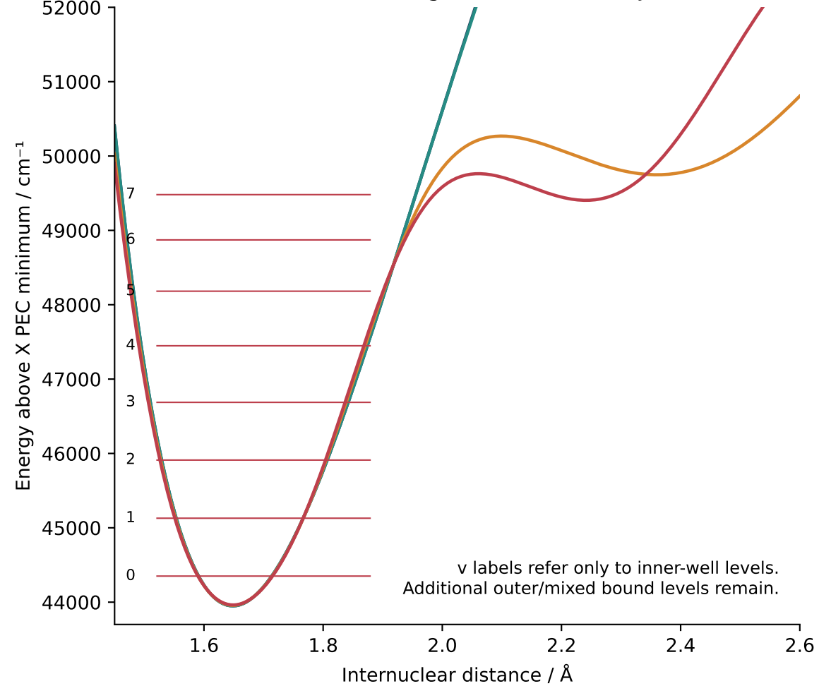
5800 \text{cm}^{-1} trial: eight inner levels at J = 1
