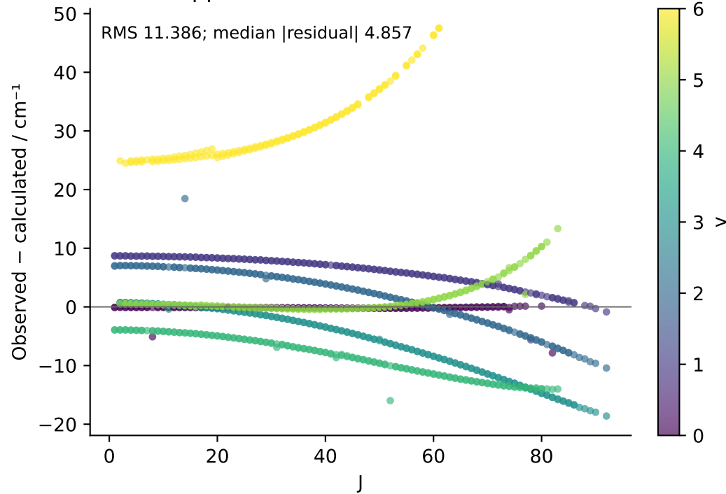
Approx. 0.78 eV above minimum
