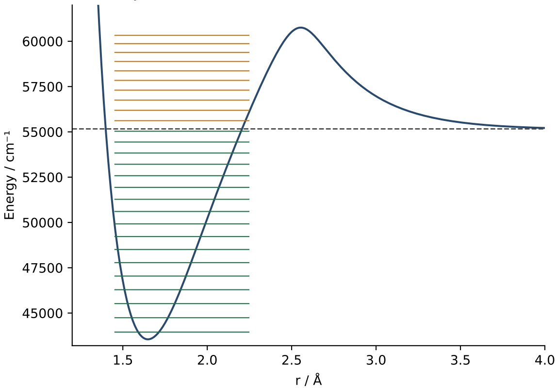
J = 1 : 17 inner bound + localized candidates
