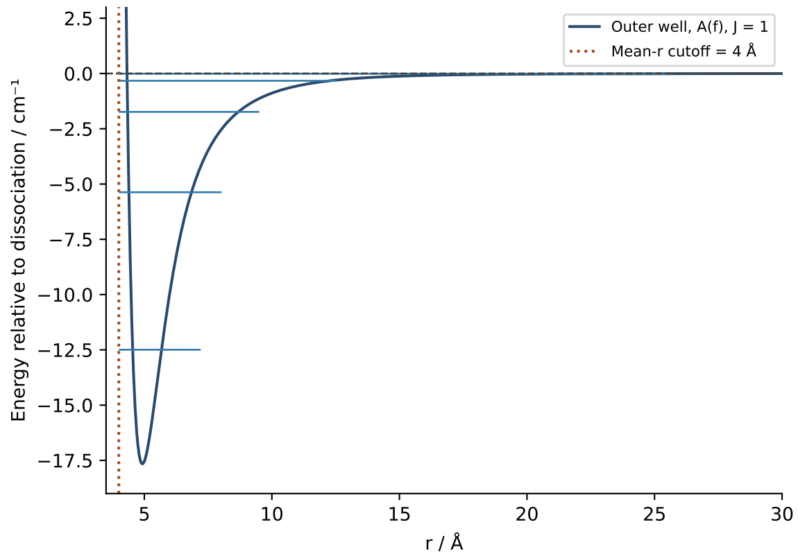
Outer bound levels fail the localization cutoff
