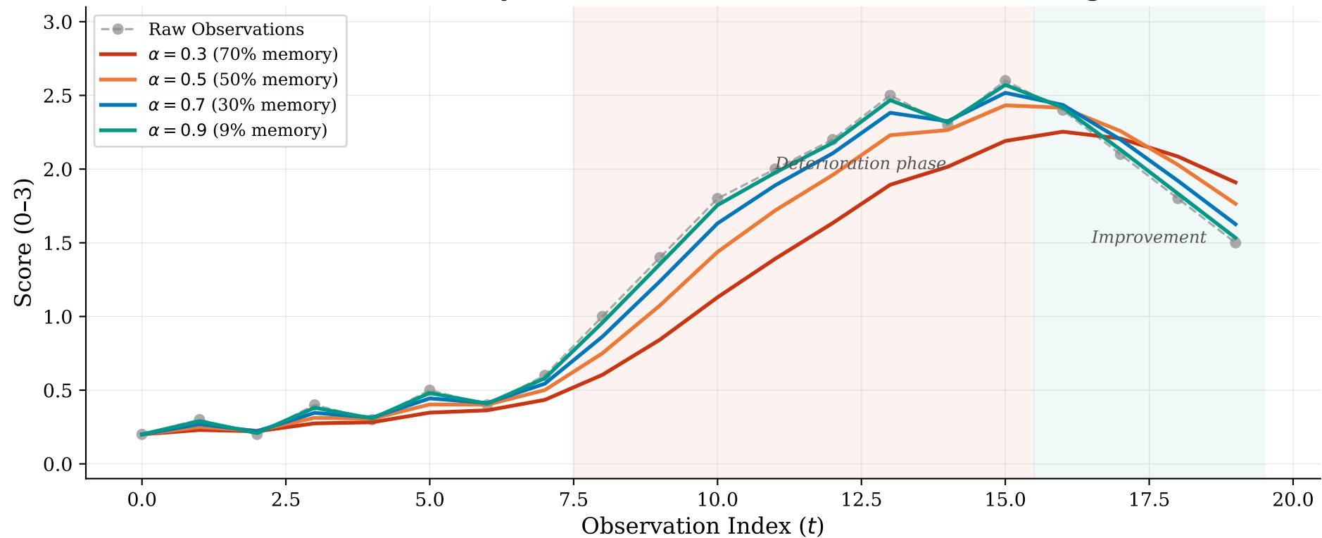
EWMA Memory Retention: Effect of \alpha on Score Smoothing
