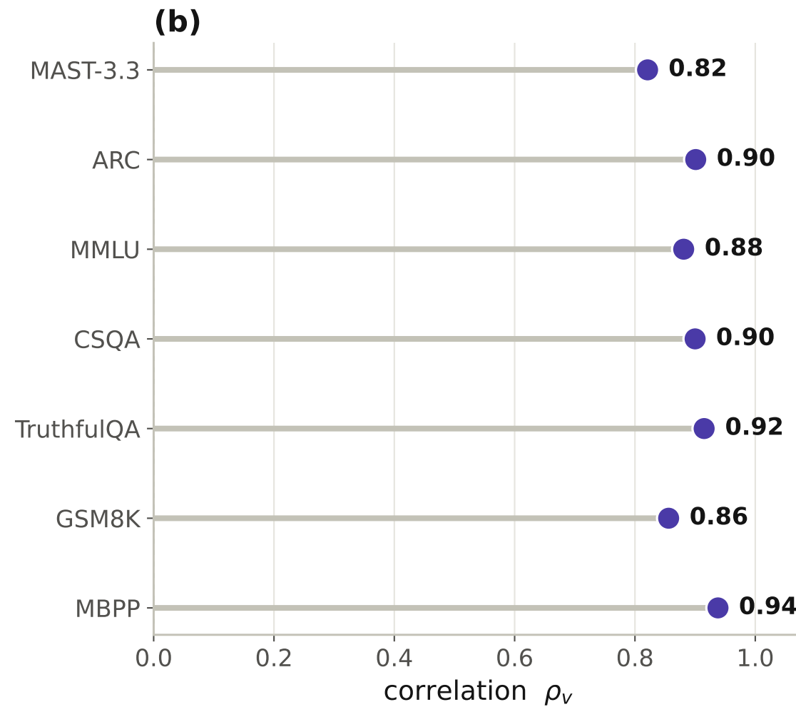
Figure 13 Same-model redundancy replicates across seven families
