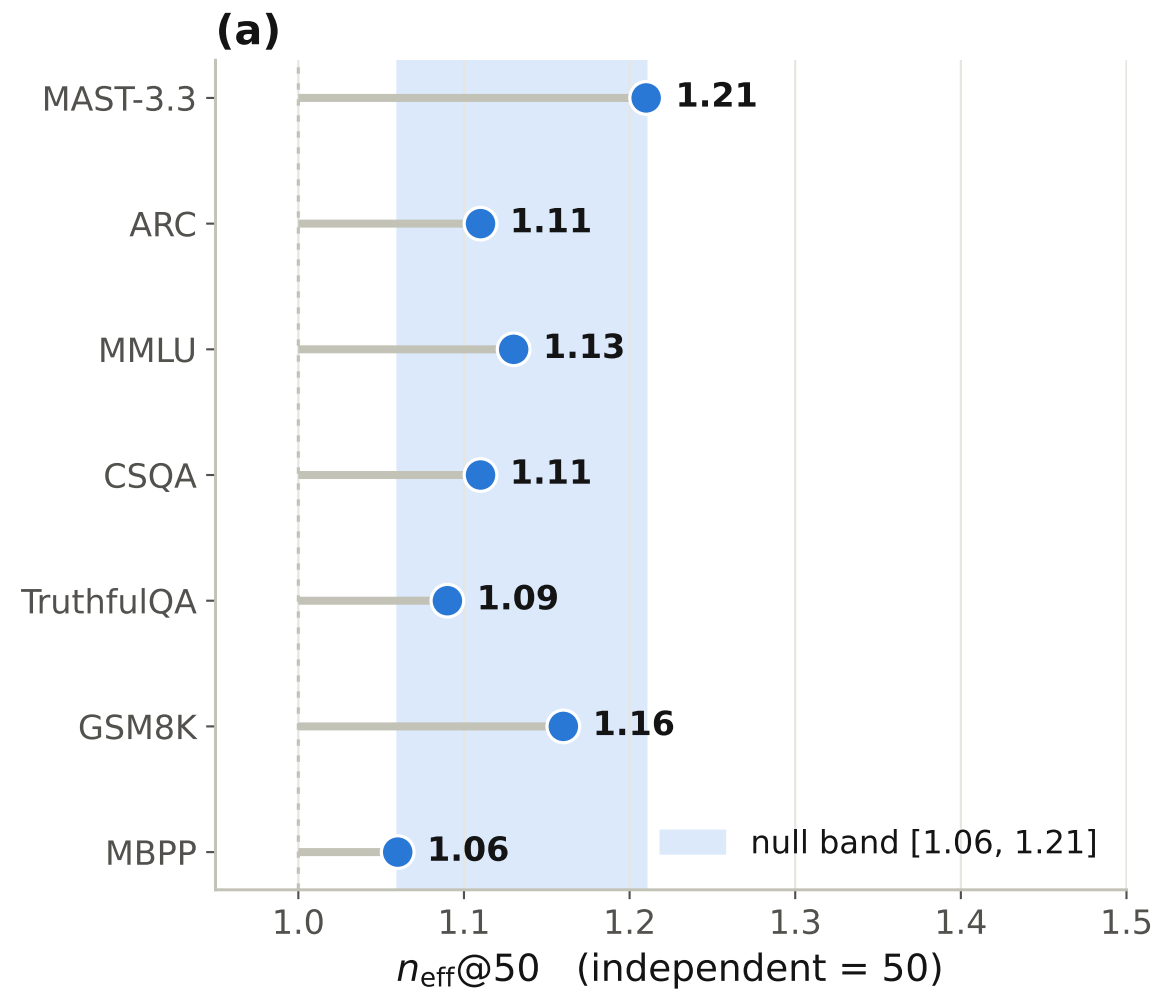
Figure 13 Same-model redundancy replicates across seven families
