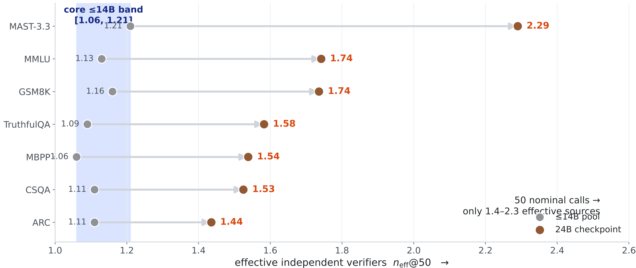
Figure 6 Redundancy persists beyond 14B — the magnitude shifts with the checkpoint
