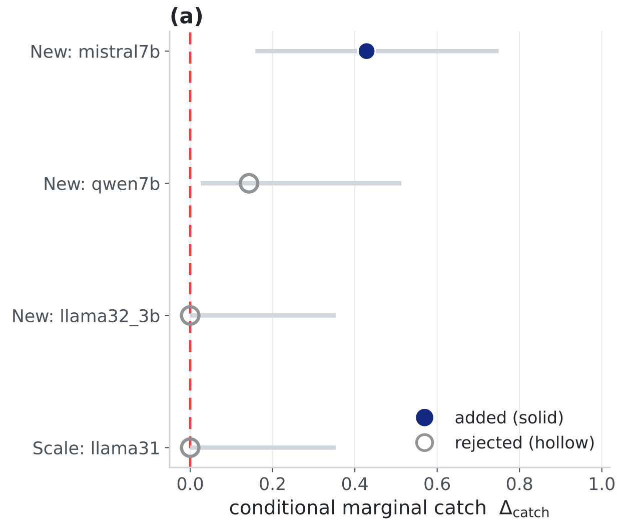
Figure 5 Conditional marginal value selects complementary verifiers
