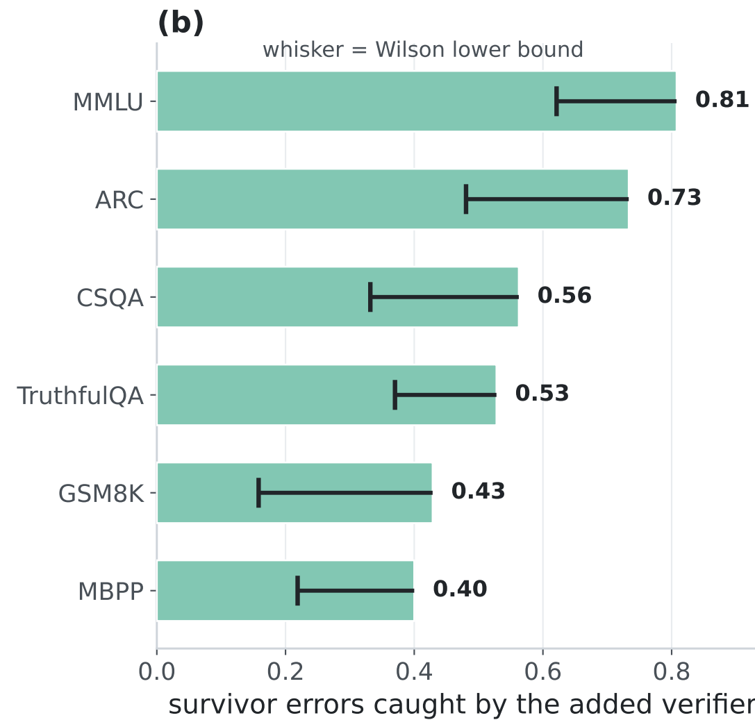
Figure 5 Conditional marginal value selects complementary verifiers
