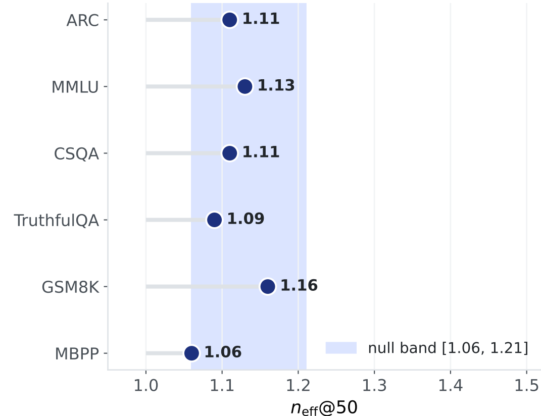
(c) Effective verifiers n_{\text{eff}}@50
