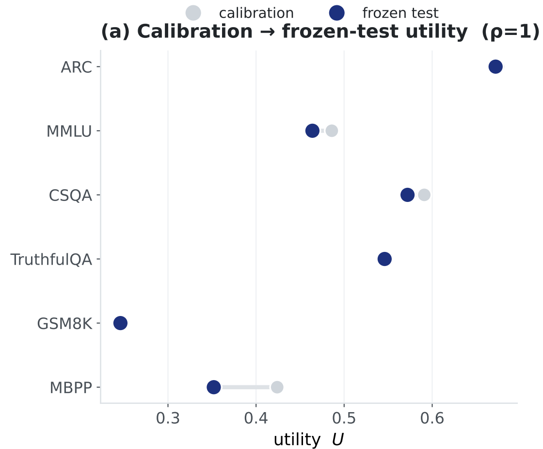
Figure B. Calibration \rightarrow frozen-test generalization
