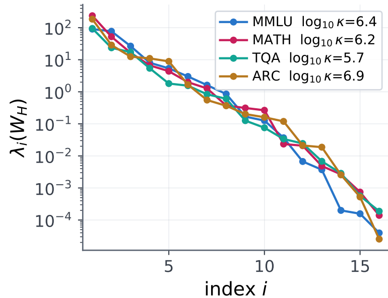
(c) Llama-3.1-8B
