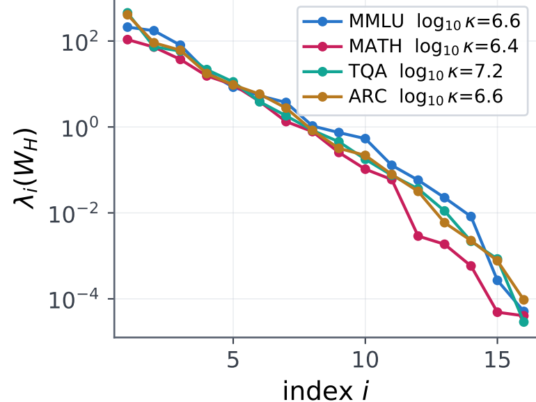
(c) Llama-3.1-8B
