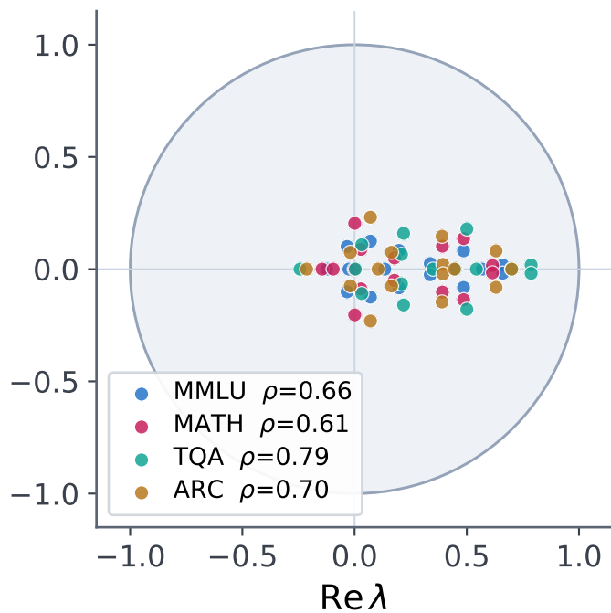
(c) Llama-3.1-8B
