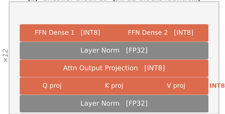
(b) Encoder Block L0 (all 12 blocks identical)
