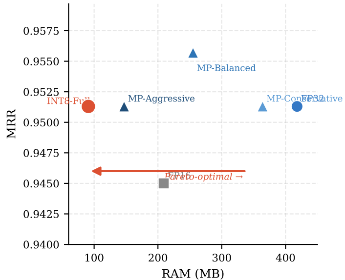
(b) RAM vs. MRR
