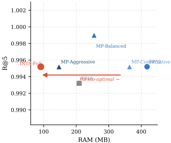
(a) RAM vs. R@5
