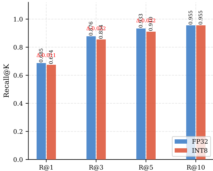
Spider 2.0-Lite (n=89 queries)
