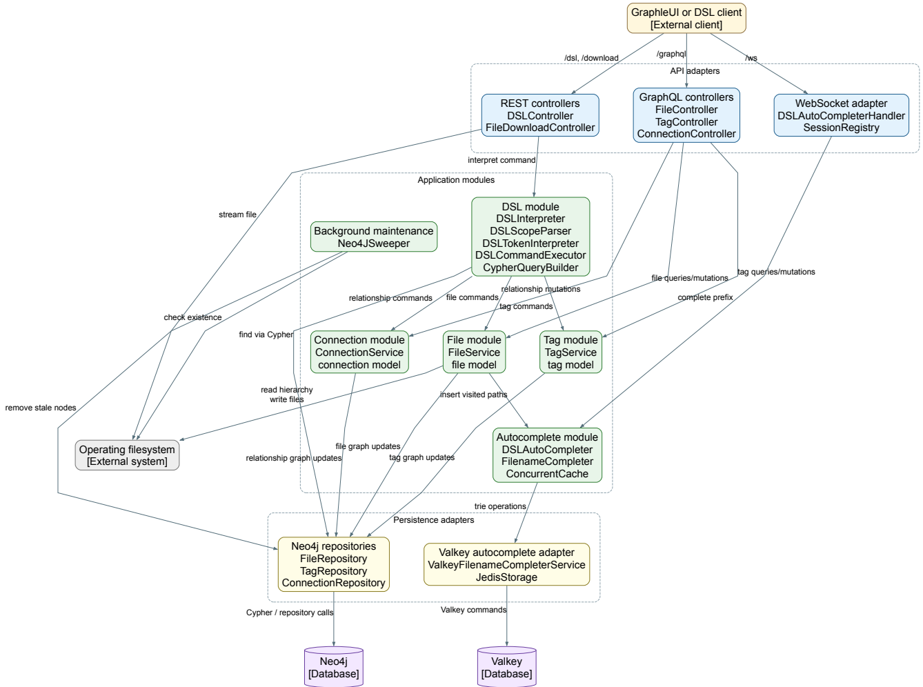
Figure 17: C4 component diagram of GraphleManager
