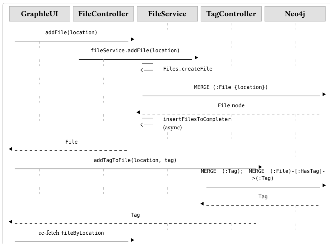
Figure 18: Adding a file and attaching a tag.
