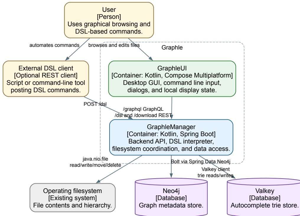
Figure 16: C4 container diagram
