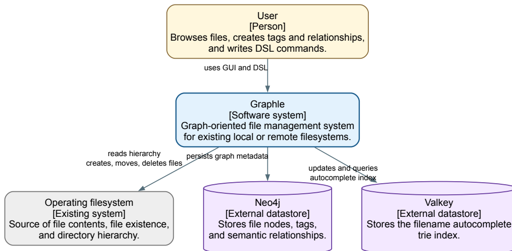
Figure 15: C4 system context diagram
