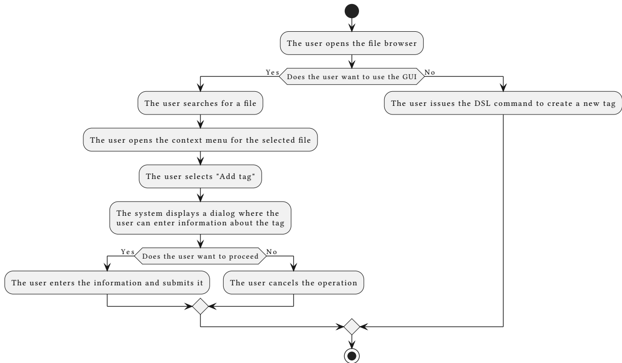
Figure 10: Add a tag activity diagram
