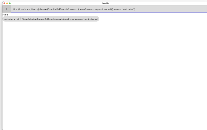
Figure 29: Main page - find results with relationship filter view
