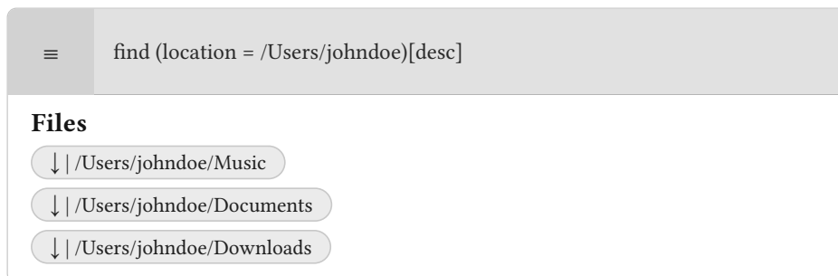
Figure 25: Main page - find results with relationship filter view
