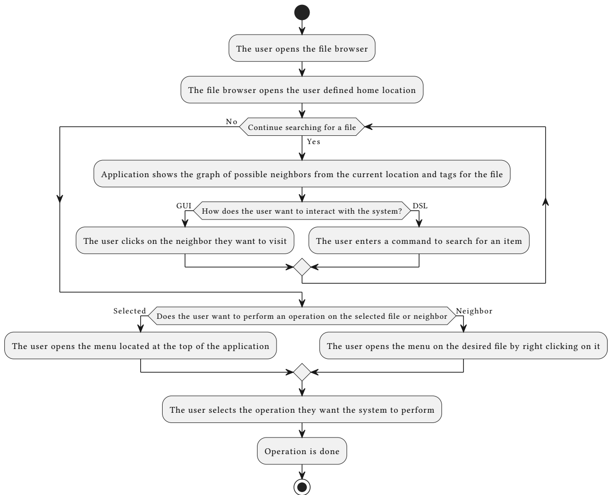
Figure 2: Search for a file activity diagram
