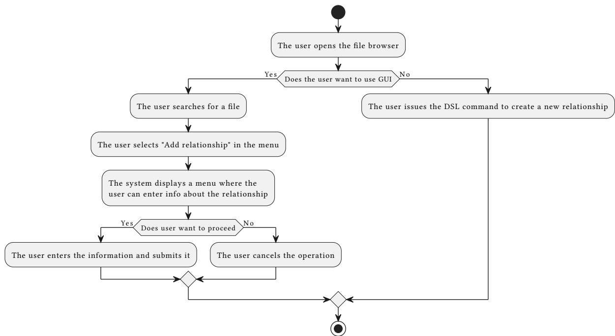
Figure 4: Add a relationship activity diagram
