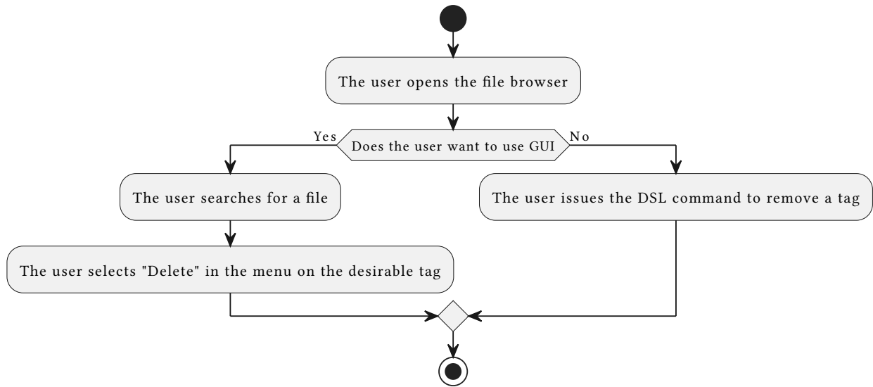
Figure 7: Remove a tag activity diagram
