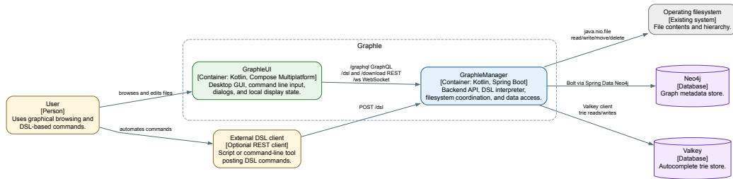
Figure 12: C4 container diagram
