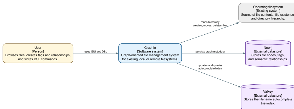
Figure 11: C4 system context diagram
