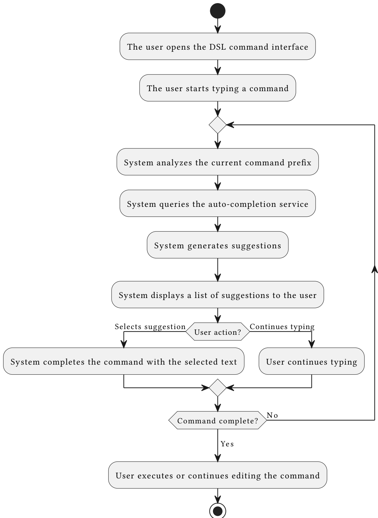
Figure 9: Command auto-completion activity diagram
