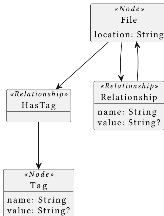
Figure 10: Graphle graph data model
