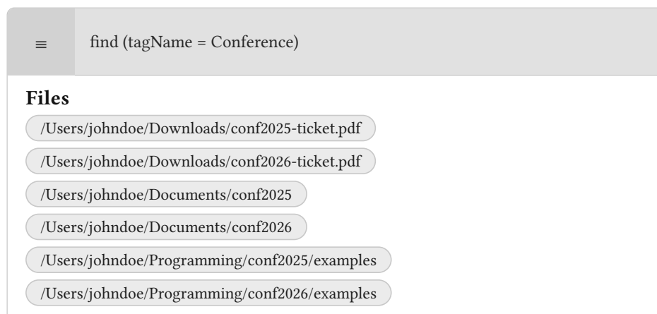
Figure 16: Main page - filenames view
