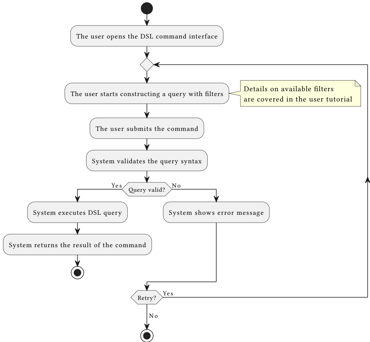
Figure 8: Complex DSL query construction activity diagram
