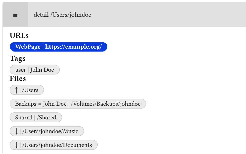
Figure 15: Main page - file detail view
