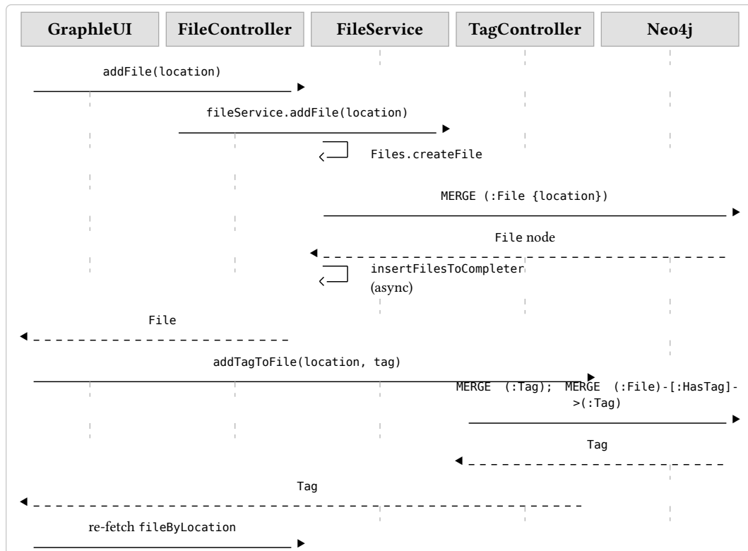
Figure 19: Adding a file and attaching a tag.
