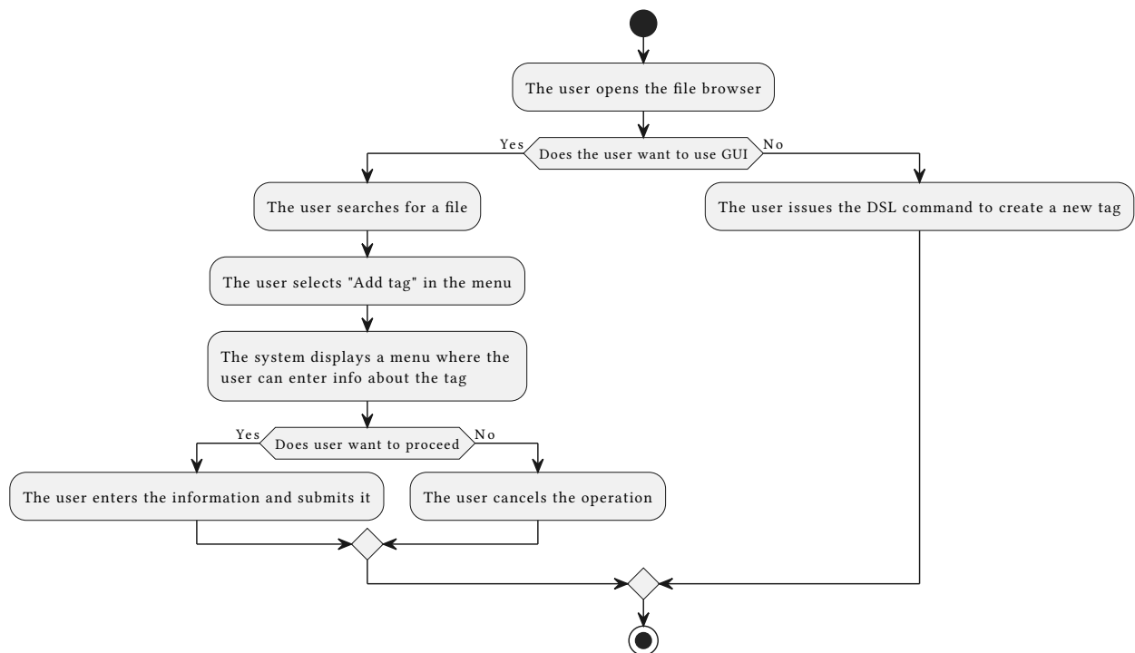
Figure 6: Add a tag activity diagram
