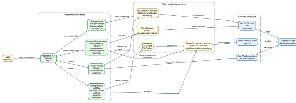
Figure 18: C4 component diagram of GraphleUI
