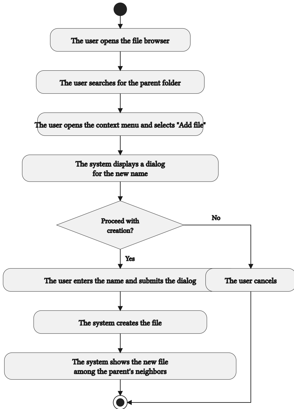
Figure 3: Create a file activity diagram
