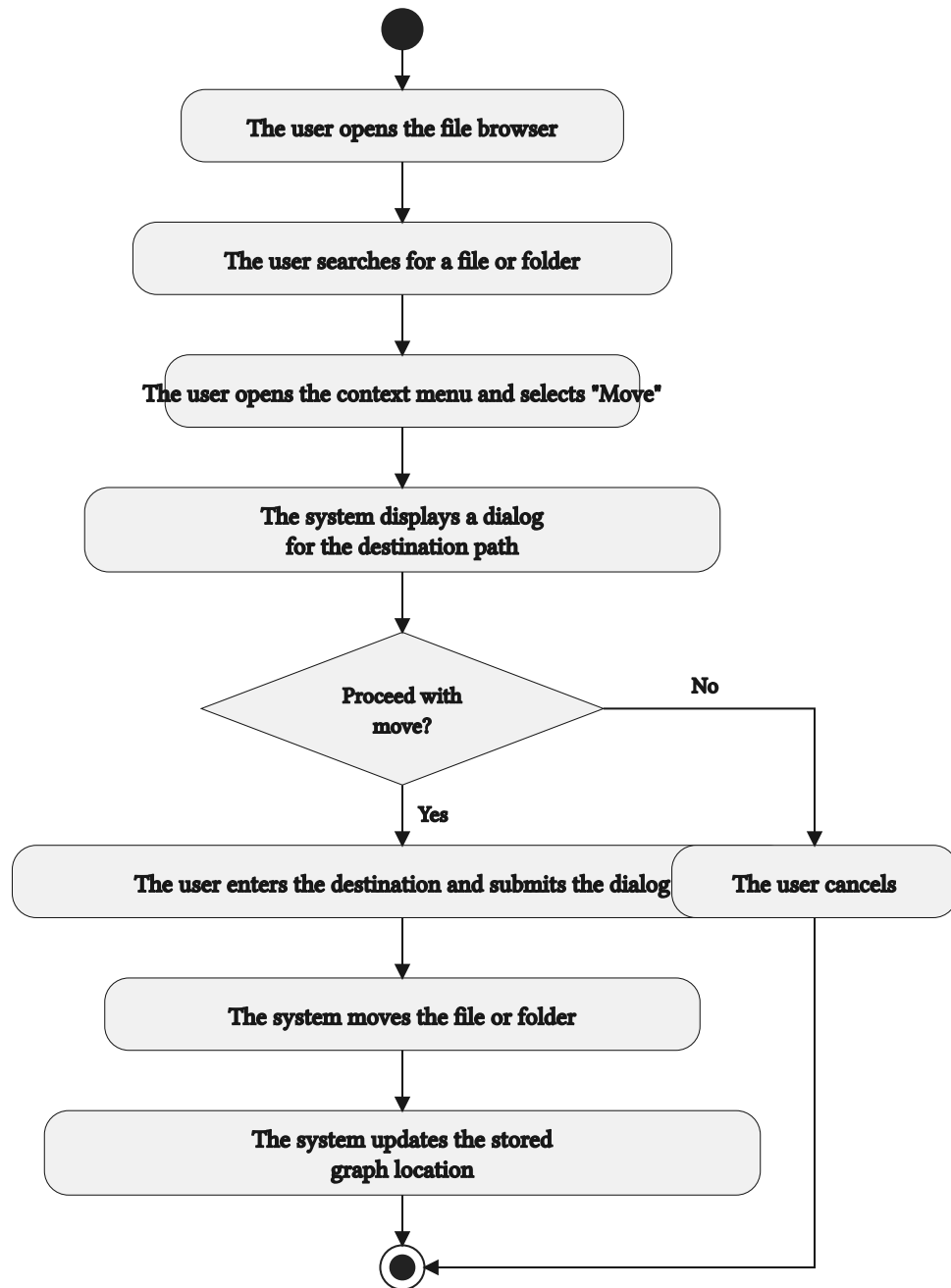
Figure 5: Move a file activity diagram
