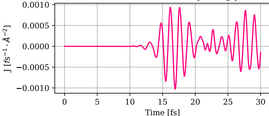
Δ matter current density along y
