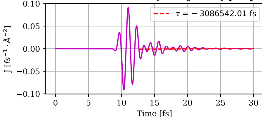
Δ energy transfer per unit cell along x
