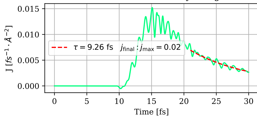
Δ matter current density along y
