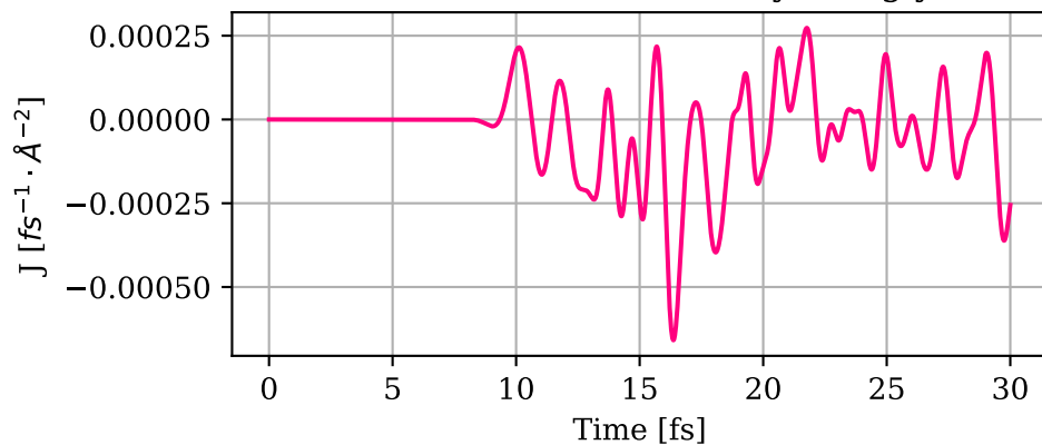
\Delta matter current density along y
