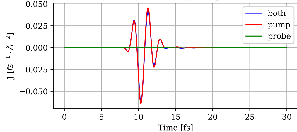
Matter current density along the z-axis
