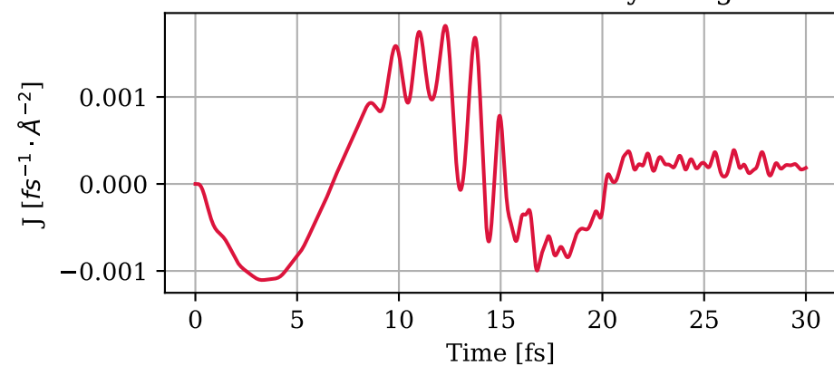
1e-5 Full matter current density along y
