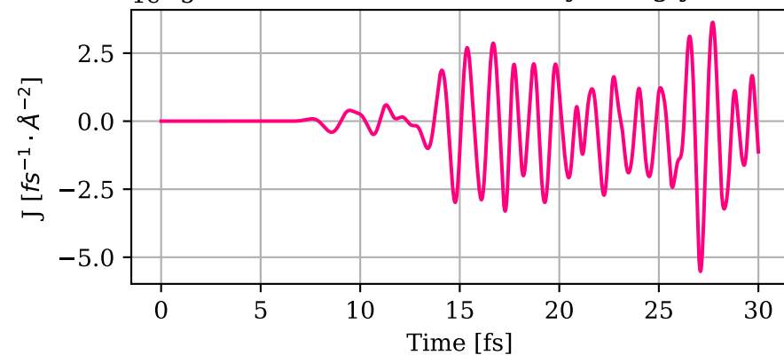
1e-5 Δ matter current density along y
