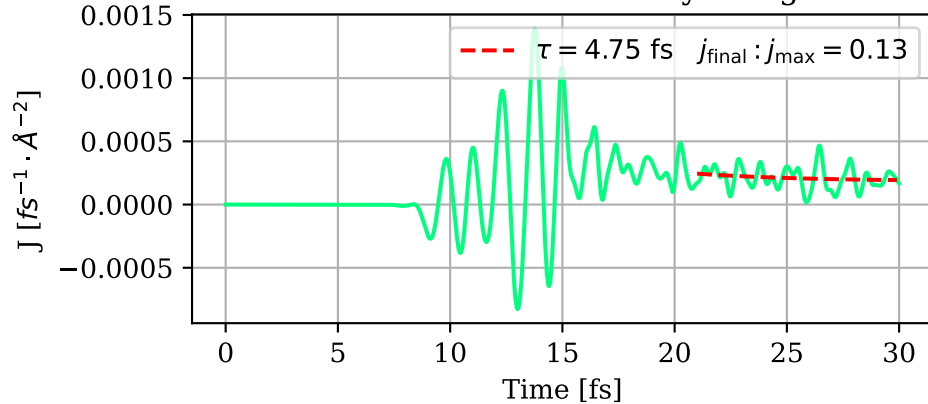
1e-5 Δ matter current density along y
