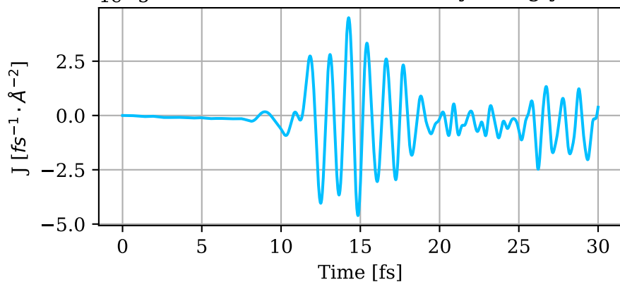
1e-5 Full matter current density along y
