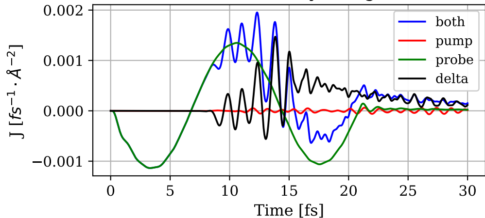
Matter current density along the x-axis
