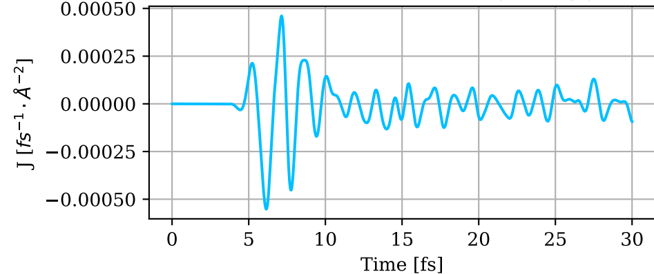
Full matter current density along y
