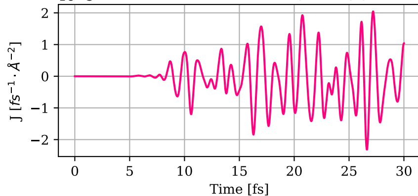
\Delta matter current density along y
