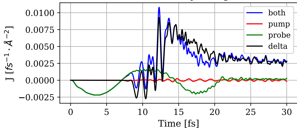
Matter current density along the x-axis
