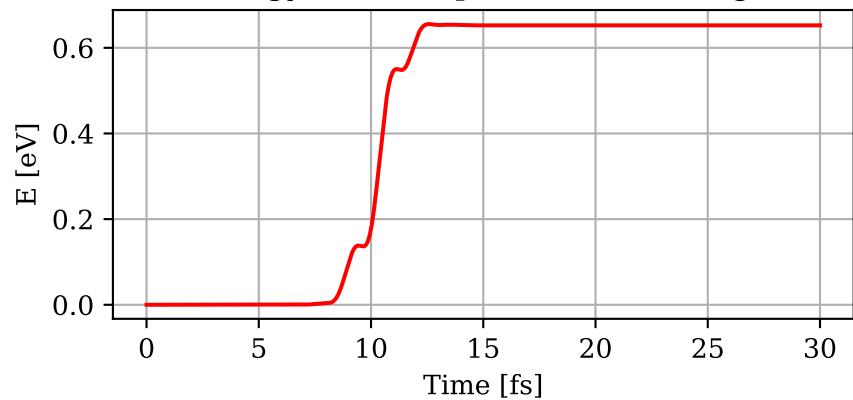
Energy transfer per unit cell along x
