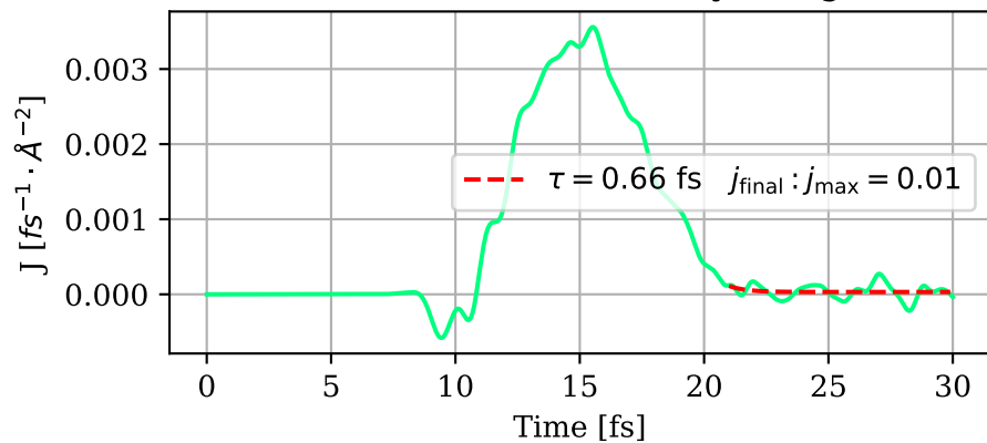
\Delta matter current density along y
