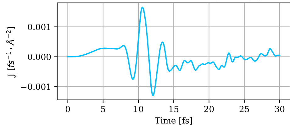
Full matter current density along y
