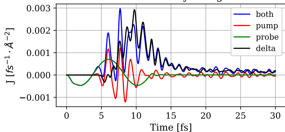
Matter current density along the x-axis
