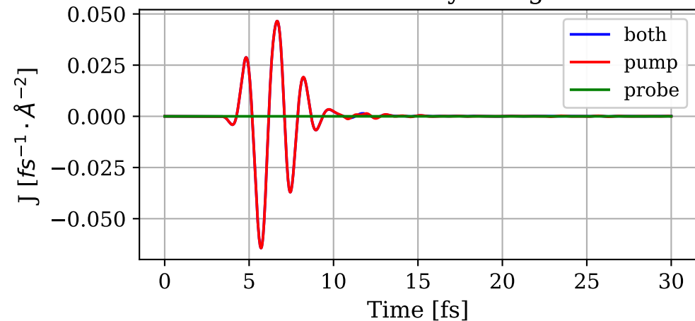
Matter current density along the z-axis
