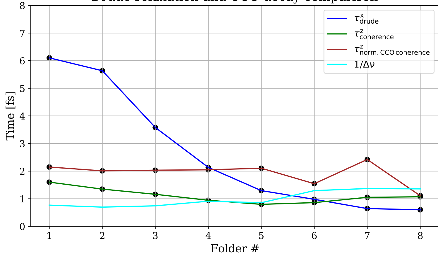
Drude relaxation and CCO decay comparison
