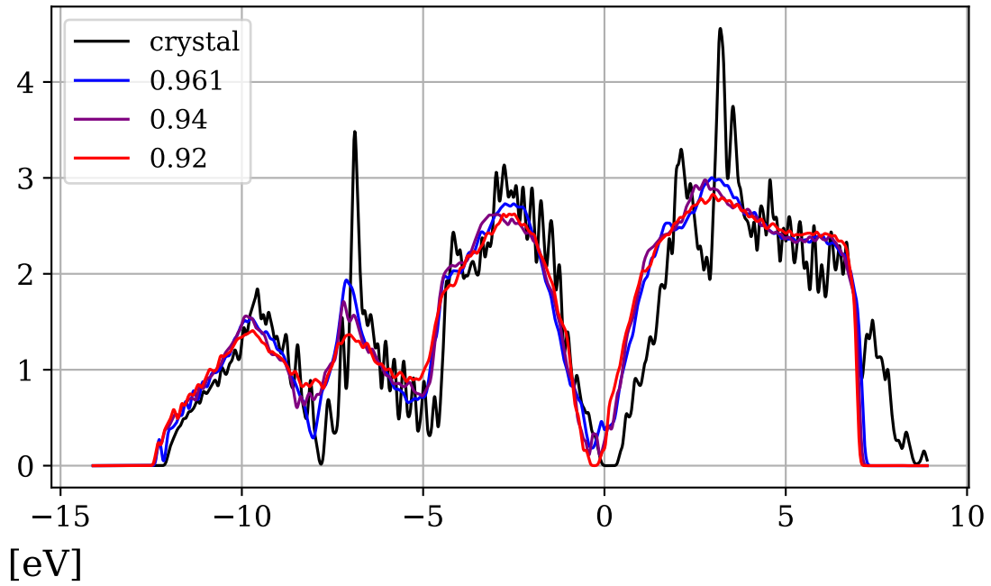
Amorphous disorder
