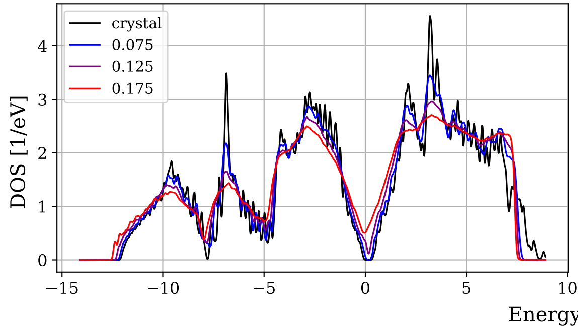
Displacement disorder
