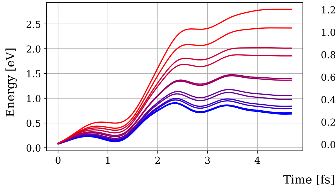
1 eV: \sigma = 4\%
