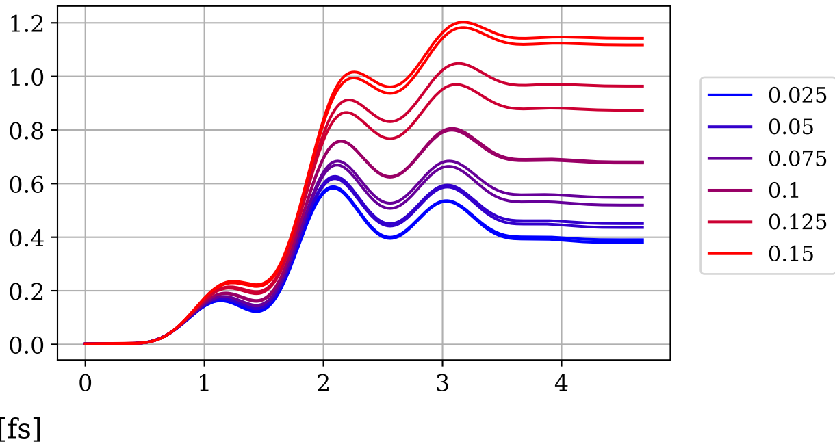
1.5 eV: \sigma = 3.5\%
